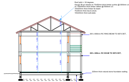
SECTION 02-02
