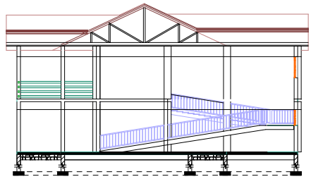
SECTION 01-01
